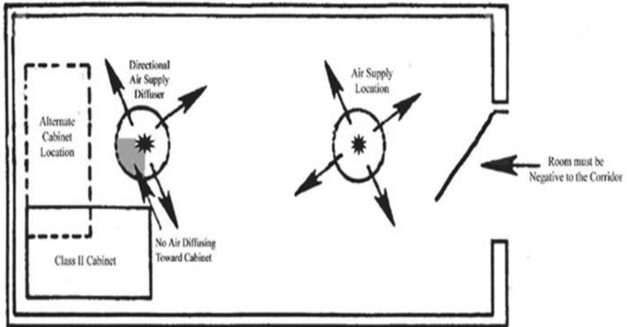
Recommended Laboratory Location for a Class II, Laminar Flow Biosafety Cabinet
